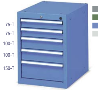
ORD. NO. DRAWERS F DA 1050 53 04 5 Cabinet with 5 full extension drawers Dim. mm 428x600x600 h Central lock
