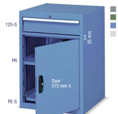
ORD. NO. DRAWERS F DD 1272 51 04 1 Cabinet with 1 normal extension drawer 1 adjustable shelf, 1 normal retractable shelf Dim. mm 564x726x825 h Central lock
